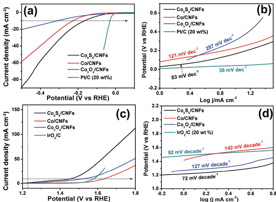
Figure 4. Electrocatalytic performance of the as-prepared self-supported nanomaterials for HER in acid and OER in alkane. a) The polarization curves of the Co 9 S 8 /CNFs, Co/CNFs, Co 3 O 4 /CNFs, and Pt/C electrocatalysts obtained in 0.5 M H 2 SO 4 with a scan rate of 2 mV s -1 . b) The corresponding Tafel slopes of the Co 9 S 8 /CNFs, Co/CNFs, Co 3 O 4 /CNFs, and Pt/C electrocatalysts. c) The polarization curves of the Co 9 S 8 /CNFs, Co/CNFs, Co 3 O 4 /CNFs, and IrO 2 /C electrocatalysts obtained in 1 M KOH with a scan rate of 2 mV s -1 . d) The corresponding Tafel slopes of the Co 9 S 8 /CNFs, Co/CNFs, Co 3 O 4 /CNFs, and IrO 2 /C electrocatalysts.
