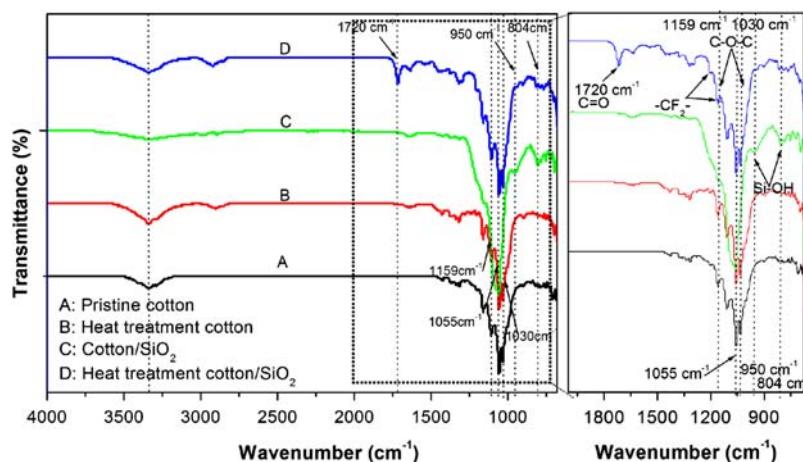
Figure 2. FT-IR spectra of pristine cotton (A), pristine cotton with heat treatment at 150°C for 10 min (B), cotton covered by SiO 2 nanoparticles with heat treatment at 150°C for 10 min (C), and the cotton fabric coated by the silica hydrosol followed by HFTMS modification and heat treatment at 150°C for 10 min (D).
