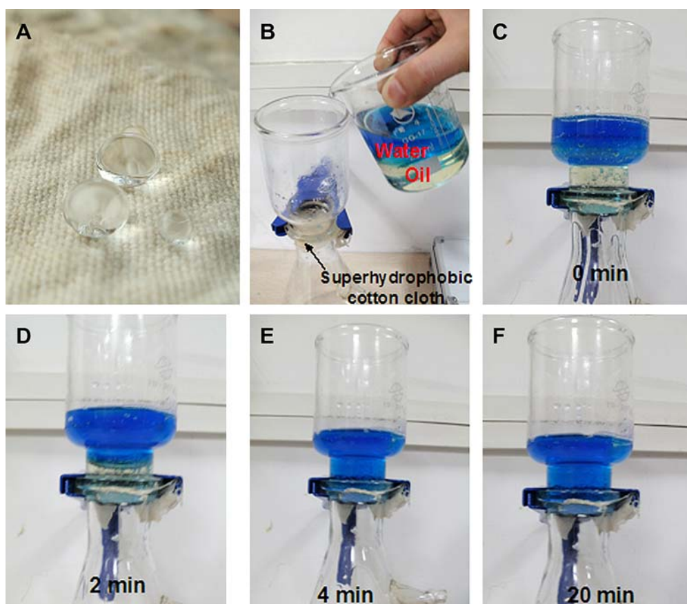
Figure 4. Optical microscope images of water droplets with different sizes on a superhydrophobic cotton cloth (A) and optical microscope images of a simple instrument for separation the mixture of oil and water (water dyed with methyl blue) (B–F).
