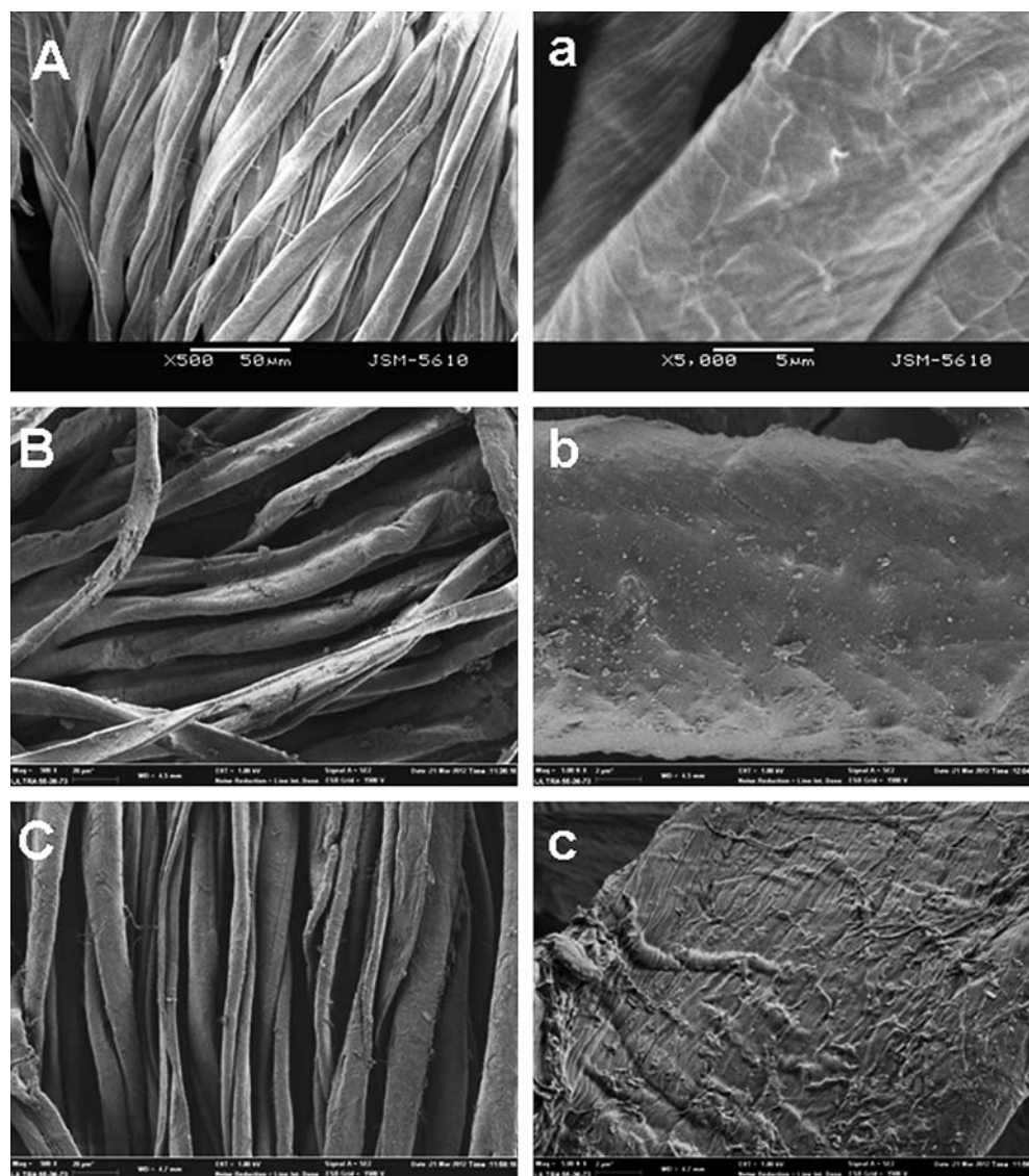
Figure 1. SEM images of (A, a) the pristine cotton fabric, (B, b) the cotton fabric coated by the silica hydrosol, and (C, c) the cotton fabric coated by the silica hydrosol followed by HFTMS modification and heat treatment at 150°C for 10 min.
