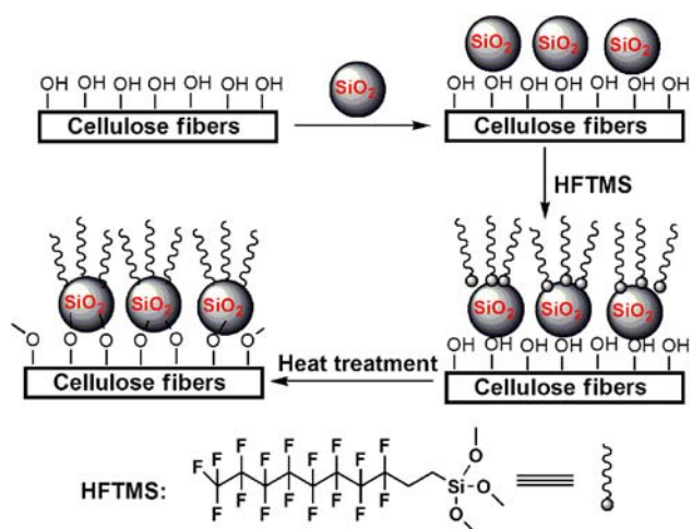
Scheme 1. Formation of superhydrophobic surfaces on cellulose fibers.
