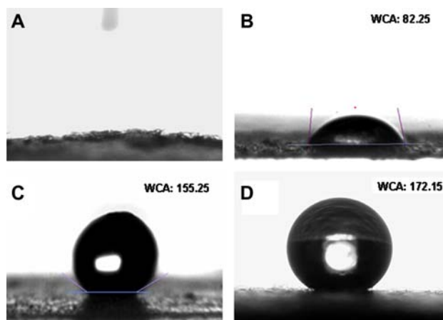
Figure 3. Water droplet (5 \mu L) images for cotton covered by SiO 2 nanoparticles (A), coated by silica hydrosols with subsequent HFTMS modification without heat treatment (B), coated by silica hydrosols with subsequent HFTMS modification and heat treatment at 100°C for 10 min (C), and coated by silica hydrosols with subsequent HFTMS modification and heat treatment at 150°C for 10 min (D).
